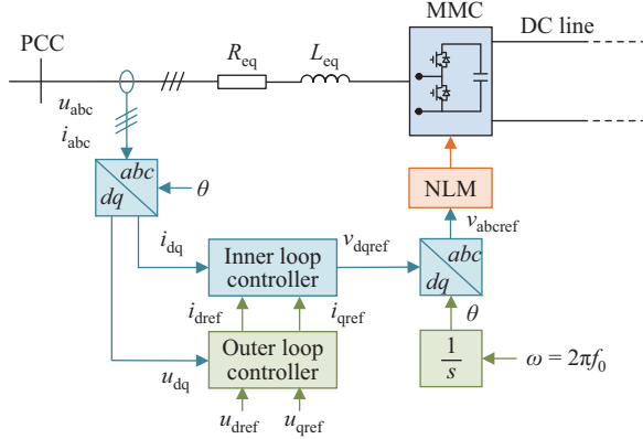
Fig. 3. The traditional control diagram of converter station S_1 .
