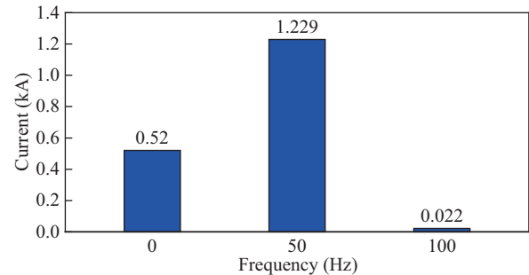
Fig. 21. Fast Fourier transform results of arm current.
